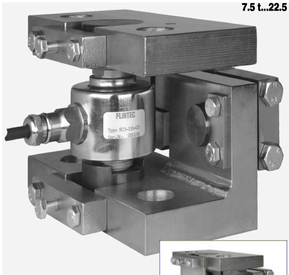
Weigh Module 55-01-11 with RC3 Load Cell
